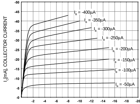
Figure 1. Static Characteristic
